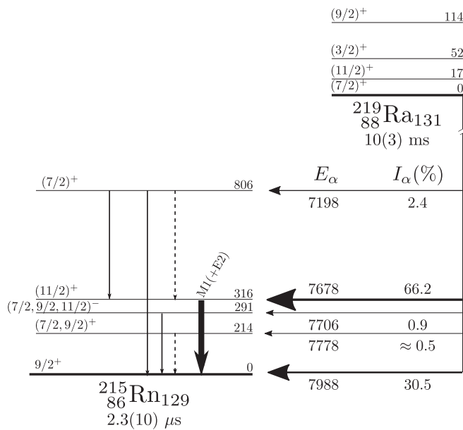
FIG. 1. Decay scheme of ^{219}\text{Ra} \rightarrow ^{215}\text{Rn} adopted from Refs. [3–5]. Level energy labels are in keV and \alpha -energies in MeV. The widths of the arrows indicate the intensity of the transition and dashed lines show tentative transitions. The ^{219}\text{Ra} levels are based on Refs. [10,12,13]. The \alpha -decay scheme is based on Refs. [1,6,7].
