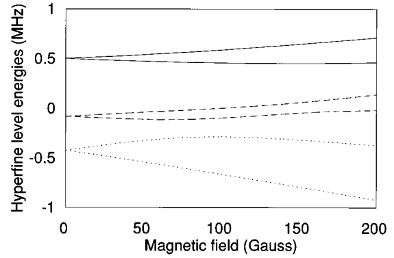
FIG. 6. Sample calculation of the Al hyperfine sublevel energies versus magnetic field. The magnetic field is oriented parallel to the c axis. |m_l| = \frac{5}{2} (solid lines), |m_l| = \frac{3}{2} (dashed lines), |m_l| = \frac{1}{2} (dotted lines).
