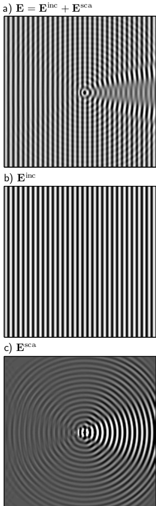
Figure 2.1. An FDTD simulation of electromagnetic wave propagation in 2 dimensions. The real part of the electric field is shown (the intensity scale is optimized for each subfigure) for the incoming field \mathbf{E}^{\text{inc}} , a plane monochromatic wave propagating from left to right and the field in presence of a small circular scatterer \mathbf{E} . The scattered field, \mathbf{E}^{\text{sca}} = \mathbf{E} - \mathbf{E}^{\text{inc}} is also shown, showing a spherical wave propagating outwards from the scatterer with intensity varying with the direction. Modified from [20].
