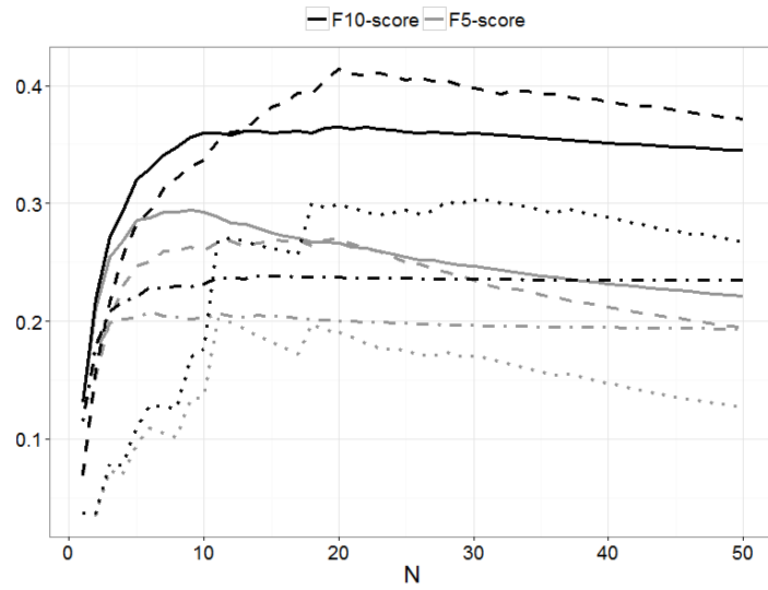
Figure 5: F-scores from the static validation, i.e., the in silico simulation. Solid line: ImpRec A, dashed line: ImpRec B, dot-dashed line: ImpRec Text, and dotted line: ImpRec Cent.
