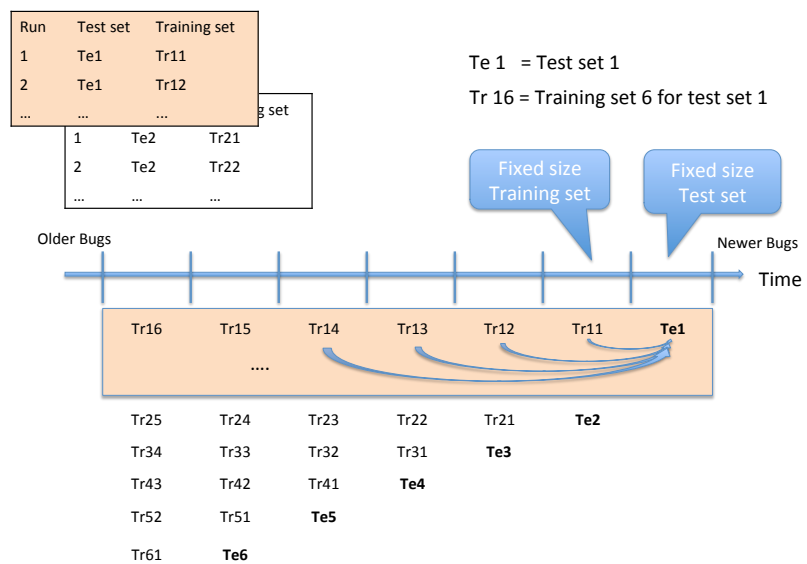
Figure 5: Overview of the time-sorted evaluation. Vertical bars show how we split the chronologically ordered data set into training and test sets. This approach gives us many measurement points in time per test set size. Observe that the time between the different sets can vary due to non-uniform bug report inflow but the number of bug reports between each vertical bar is fixed.
