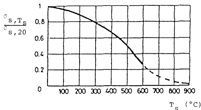
Figure 14 : Quotient between effective yield stress \sigma_{s,T_s} at elevated temperature T_s and yield stress at room temperature as a function of steel temperature T_s . The curve applies to steel grades Fe 360 to Fe 510 with an accuracy, which is sufficient for practical purposes (11)
