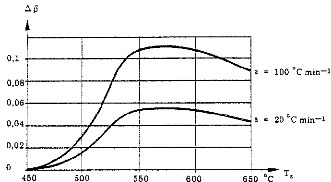
Figure 12 : Increase \Delta\beta of coefficient \beta determined according to fig. 11, for a rate of heating a \geq 4^\circ\text{C. min}^{-1} , as a function of the steel beam temperature T_s (8), (20).
