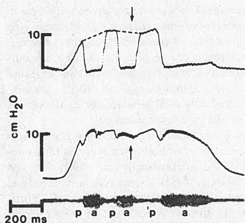
FIG. 1. Simultaneous records of oral pressure (top), subglottal pressure (middle), and audio signal (bottom) during production of the nonsense syllables 'papa'pa. The pressure signals have been low-pass filtered at 70 Hz. The broken line in the oral pressure curve illustrates the method of linear interpolation between the pressures associated with the voiceless stops in order to get an estimate of subglottal pressure during the vowels between the voiceless consonants. The arrows indicate the point during the utterance at which the measurement was made of direct and indirect subglottal pressure.
