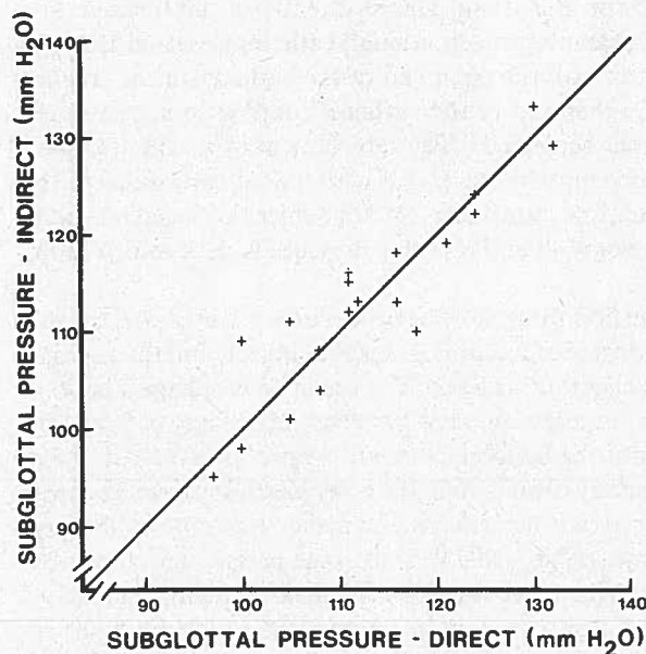
FIG. 2. Plot of direct and indirect measurements of subglottal pressure ( n = 20 ).
