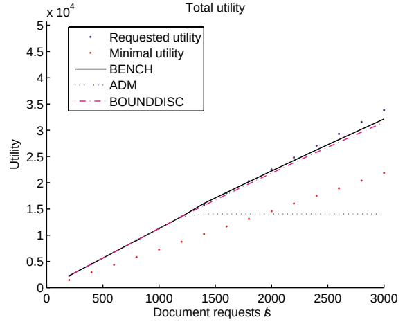
Figure 3: Utility of the different solutions.
