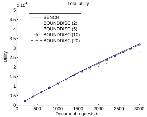
Figure 4: Obtained utility using solution given 2, 5, 10 and 20 possible byte counts ( BOUNDDISC solution), compared to the BENCH solution.
