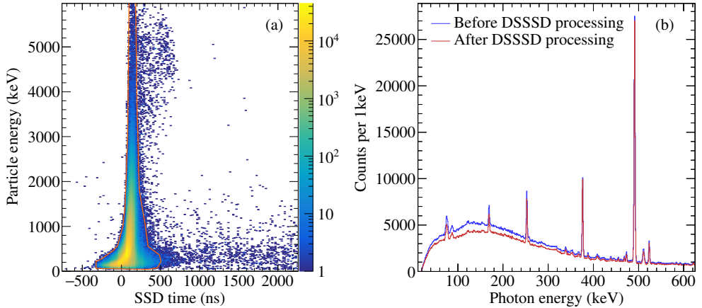
Figure 3.2: (a) Correlation between the energy and time of charged particles detected with the DSSSDs during the ^{127}\text{Cd} experiment as well as the gate condition to reduce random background. (b) Resulting improvement on the photon spectrum in prompt coincidence with a charged particle after applying the gate condition seen in panel (a), inter-strip add-back and requiring matching pairs of p-side and n-side signals.
