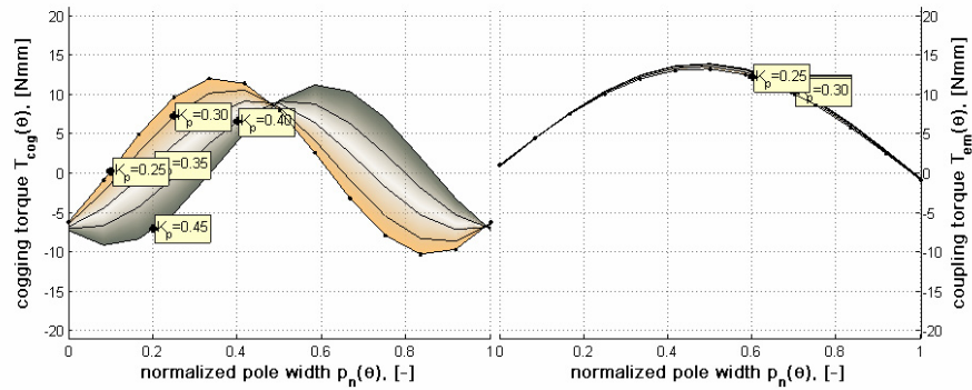
Figure 5.5: The angular pole width influence on the static characteristics of the single-phase claw-pole motor ( \gamma_l=30^\circ ) when the axial air-gap is present ( g_s=0.15 mm).
