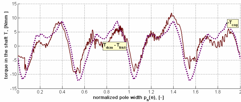
Figure 5.44 Static core loss measurement, torque characteristics over one mechanic revolution at low magnetization frequency of 0.07 Hz. The sum of magnetization friction and cogging torque (solid line) is compared to the inverted static torque measurement (dotted line) that is obtained from weighting-scale method.
