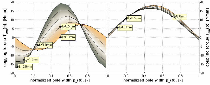
Figure 5.14: The progressive radius influence of the static characteristics of the single-phase claw-pole motor. The shape of the claw-pole is determined by tangential tapering \gamma_t = 8^\circ and pole clearance factor K_p = 0.38 .
