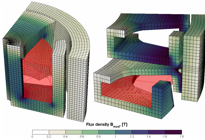
Figure 4.2: Magnetic loading of polar magnet motors.
