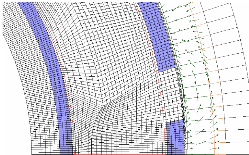
Figure C.3: 3D FE mesh in the radial/circumferential plane of the two-phase claw-pole motor.
