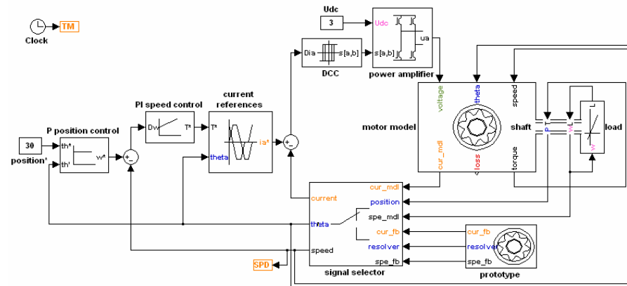
The control system is made in such a way that it is able to use a motor model or the real prototype motor. The selection of the feedback signal is made in a signal selector block.
