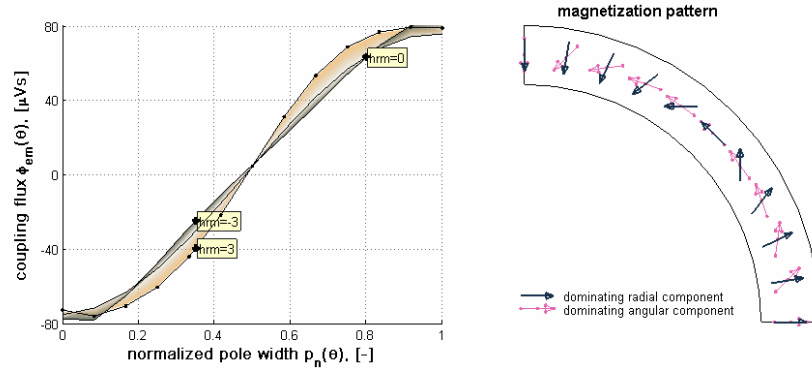
Figure 5.28: Third harmonic (3rm) introduced in the permanent magnet excitation field (right), and the corresponding coupling flux waveform in the centre core (left).
