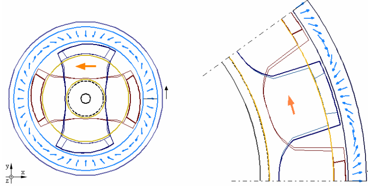
Figure 5.1: Specification of the negative current flow direction (big arrow on the winding domain), magnetization vectors (vectors in the magnet-ring region) and the direction of the motion (small dark arrow outside of the outer rotor) on the top view of the claw-pole motors in xy -plane. The rotor is turned from the initial alignment (0) to the next alignment position (1) of the same phase.
