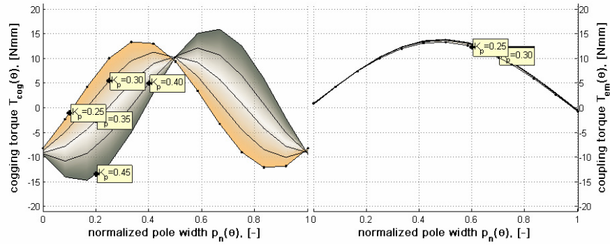
Figure 5.4: The angular pole width influence on the static characteristics of the single-phase claw-pole motor ( \gamma_l=0^\circ ) when the axial air-gap is present ( g_s=0.15 mm).
