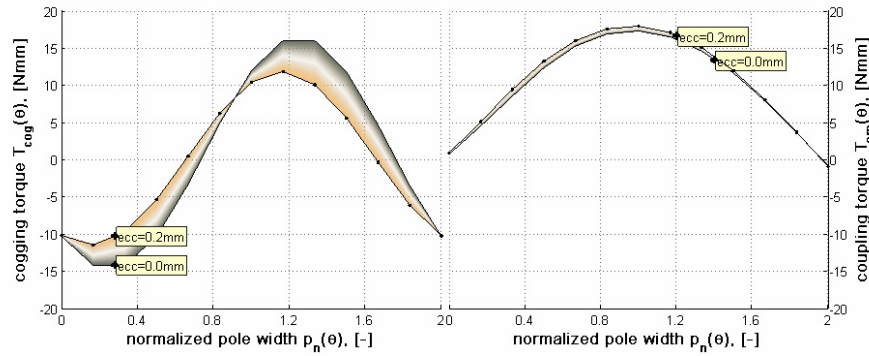
Figure 5.17: Influence of the static rotor eccentricity ( ecc ) on motor torque characteristics.
