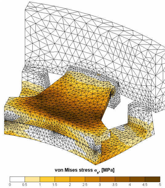
Figure 4.14: Mechanical stresses in a claw-pole ring of the two-phase claw-pole motor due to the rotor assembling.
