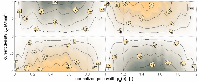
Figure 6.1: The current density needed to produce electromagnetic torque. The equi-torque contours ( T_{em} in Nmm ) show the corresponding electromagnetic torque as a function of rotor position and current. The initial zero position is at alignment position of the magnet pole and the claw-pole.
