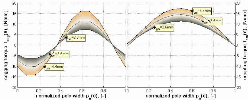
Figure 5.27: The thickness of the magnet-ring l_{pm} influences the static characteristics of the single-phase claw-pole motor. The shape of the claw-pole is determined by tangential tapering \gamma_t=8^\circ and pole clearance factor K_p=0.38 .
