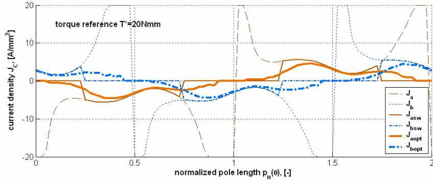
Figure 6.3: Selection of current density reference profile to produce a constant torque of 20 Nmm in the two-phase claw-pole motor. The thin lines ( J_a, J_b ) show the required current density if a single-phase has to provide the reference torque. Alternatively, the reference current can be selected according to minimized switching ( J_{asw}, J_{bsw} normal lines) or copper losses ( J_{aopt}, J_{bopt} bold lines).
