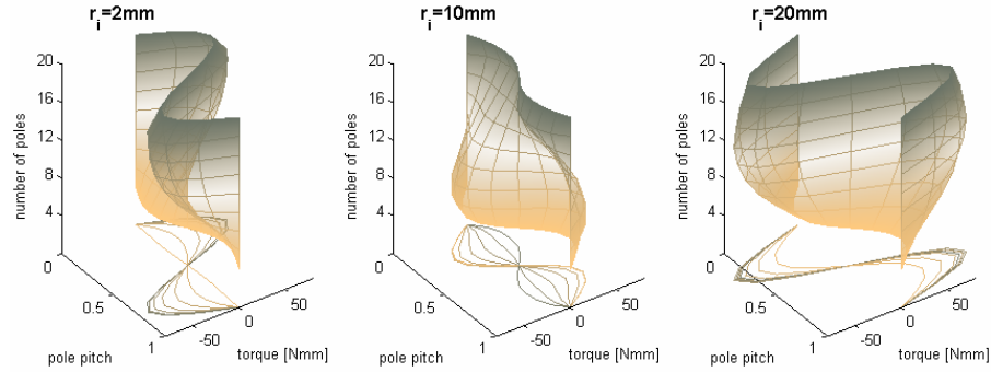
Figure 4.24: Cogging torque waveform depending on number of poles and on the air-gap radius. The air-gap radius is the result of a given inner radius and the constant volume of stator core. Depending on the coupling length through the core compared to the leakage via claw-poles the rotor has stabile equilibrium position where the coupling torque is the biggest for the symmetric poles.
