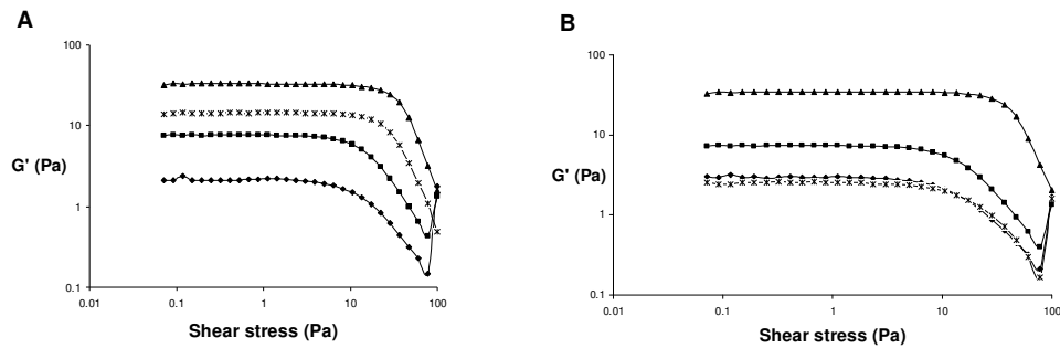
Figure 20. The elastic modulus, G' , of the continuous phase of the fibre suspensions. A) 0.8% suspensions; B) 1.2% suspensions. \diamond - apple; \times - tomato; \blacktriangle - potato pulp; \blacksquare - carrot. From Paper I.
