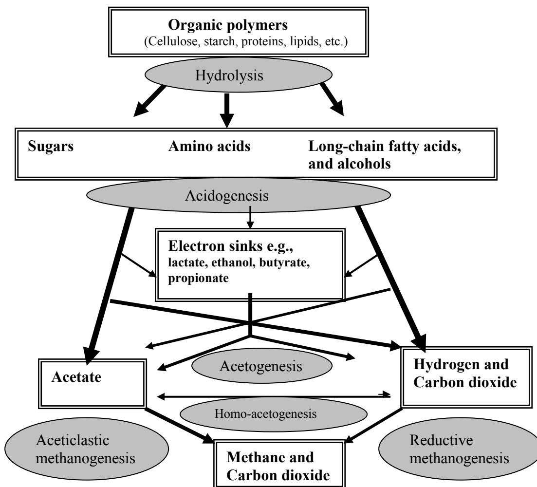
Figure 1. The main degradation pathways in anaerobic digestion
