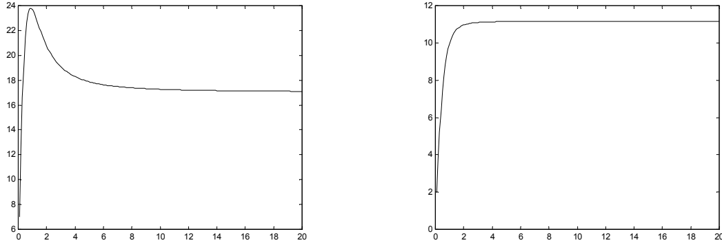
Figure A.1. Typical Log-Likelihood Functions for the Measurement Error (a) Well-Behaved Likelihood (b) Ill-Behaved Likelihood
