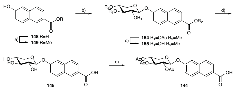
Scheme 6.3. Synthesis of xylosylated hydroxynaphthoic acids 142 and 144 as illustrated with 144 . a) \text{SOCl}_2 , MeOH, 75 °C, sealed tube, 91% (81%). b) 1,2,3,4-Tetra- O - \beta -D-xylopyranoside, \text{BF}_3 \cdot \text{OEt}_2 , \text{CH}_2\text{Cl}_2 , r.t., 83% (95%). c) NaOMe, MeOH, r.t., 97% (90%). d) NaOH, MeOH, r.t. 95% (99%). e) \text{Ac}_2\text{O} , pyridine, r.t., 90% (91%). Yields within parentheses are for the same reactions using 146 as starting material to give 142 . See the Supplementary information chapter for experimental details.
