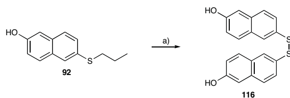
Scheme 5.7. Synthesis of hydroxynaphthyl disulphides as illustrated by 116 . a) i) \text{Na} , \text{NH}_3 , \text{Et}_2\text{O} , -33\text{ }^{\circ}\text{C} . ii) \text{I}_2 , \text{MeOH} , \text{H}_2\text{O} , r.t., 83%.
