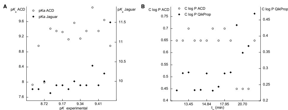
Figure 4.5. Comparison of experimentally determined pK_a values and values calculated in ACD/Labs (A) and Jaguar and experimentally determined gradient HPLC retention times and C log P values calculated in ACD/Labs and QikProp (B), showing the difficulties in prediction of physical properties by computational methods.
