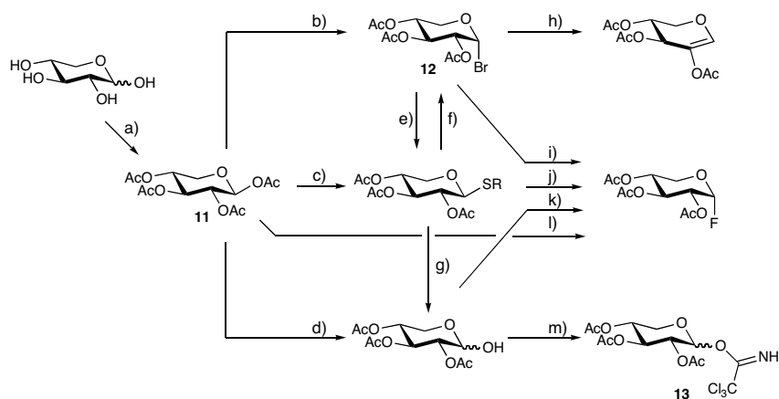
Scheme 1.3. Examples of interconversions between xylopyranoside donors. a) \text{Ac}_2\text{O} , \text{NaOAc} , 140\text{ }^\circ\text{C} , 1\text{ h} . 14 b) \text{HBr}/\text{HOAc} , \text{Ac}_2\text{O} , r.t., 1\text{ h} . 15 c) \text{RSH} , \text{BF}_3\cdot\text{OEt}_2 , \text{CH}_2\text{Cl}_2 , 0\text{ }^\circ\text{C} , 45\text{ min} . 16 d) Amine, \text{THF} , 75\text{ }^\circ\text{C} , 18\text{ h} . 17,18 e) \text{NaSPh} , \text{Et}_2\text{O} , r.t., 2\text{ d} . 19 f) \text{IBr} , \text{CH}_2\text{Cl}_2 , 0\text{ }^\circ\text{C} , 10\text{ min} . 20 g) \text{NBS} , acetone, \text{H}_2\text{O} , r.t., 1\text{ h} . 21 h) \text{Zn}/\text{Ag}-\text{C} , \text{THF} , -20\text{ }^\circ\text{C} , 10\text{ min} . 22 i) \text{AgF} , \text{CH}_3\text{CN} , r.t., 2\text{ h} . 23 j) \text{DAST} , \text{NBS} , \text{CH}_2\text{Cl}_2 , 0\text{ }^\circ\text{C} to r.t., 25\text{ min} . 24,25 k) \text{DAST} , \text{CH}_2\text{Cl}_2 , 78\text{ }^\circ\text{C} , 15\text{ min} . 25 l) \text{HF}/\text{pyridine} , 0\text{ }^\circ\text{C} , 6\text{ h} . 26 m) \text{Cl}_3\text{CCN} , \text{DBU} , \text{CH}_2\text{Cl}_2 , -10\text{ }^\circ\text{C} to r.t., 3\text{ h} . 27 Adapted from paper I.
