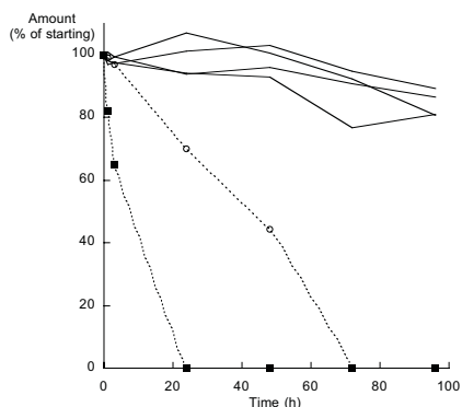
Figure 5.13. Stability profiles of hydroxynaphthyl 1-thio- \beta -D-xylopyranosides ( 80-85 ) in Ham's F-12 medium at 37 °C. The graph shows the concentration of xyloside compared to an internal standard as analysed by HPLC. Whilst 4 of the xylosides show only slight decomposition (solid lines), 80 (○) and 82 (■) decompose totally.
