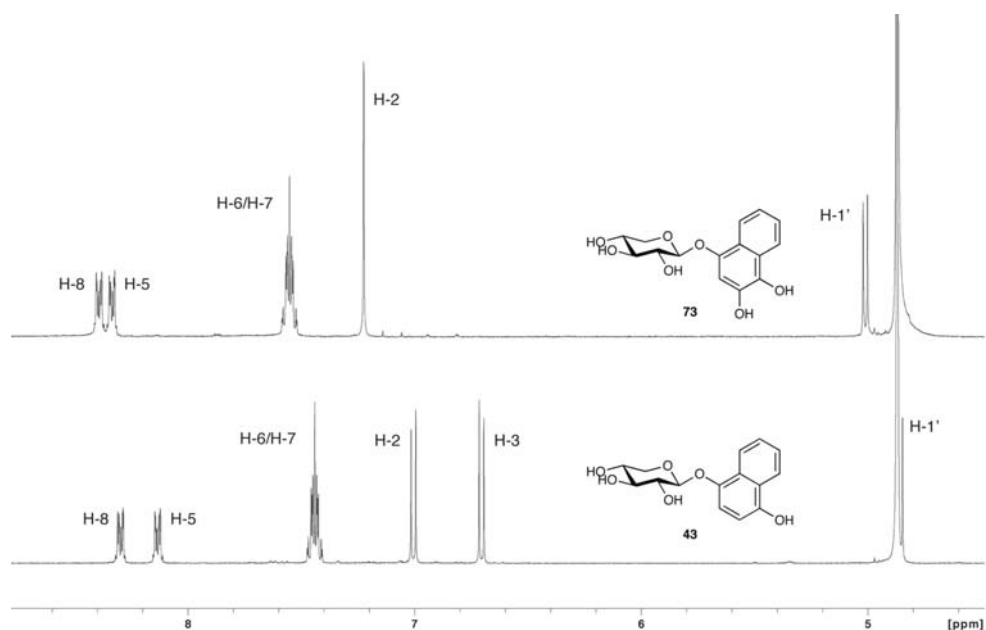
Figure 4.7. ^1\text{H-NMR} spectra of 43 (bottom trace) and 73 (top trace) showing the anomeric ( \text{H-1}' ) and aromatic proton signals.
