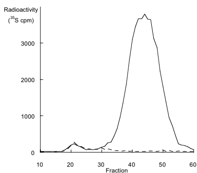
Figure 5.14. Priming of GAG chains in T24 cells treated with 84 (0.1 mM, solid line) or untreated (dashed line). Xyloside primed GAG chains elute in pool II whilst PG primed GAG chains elute in pool I.
