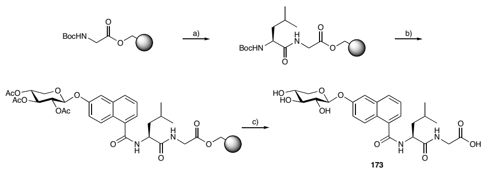
Scheme 6.6. Solid-phase synthesis of naphthyl xyloside-amino acid conjugates as illustrated using the synthesis of 173 . a) i) TFA (80% in CH 2 Cl 2 containing 0.4 M thiophenol), r.t. ii) DMAP, 159 (HCl salt), CH 2 Cl 2 , r.t. iii) DIC in CH 2 Cl 2 , r.t. b) i) TFA (80% in CH 2 Cl 2 containing 0.4 M thiophenol), r.t. ii) DMAP, 142 , CH 2 Cl 2 , r.t. iii) DIC in CH 2 Cl 2 , r.t. c) i) NaOMe, MeOH, CH 2 Cl 2 , r.t. ii) NaOH (1 M, aq.), MeOH, r.t. 61%. See the Supplementary information chapter for experimental details.
