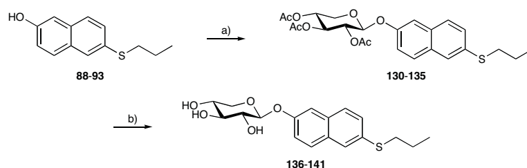
Scheme 5.10. Xylosylation of thiopropyl substituted naphthols as illustrated with 92 . a) 1,2,3,4-Tetra- O -acetyl-β-D-xylopyranoside, BF 3 •OEt 2 , Et 3 N, CH 2 Cl 2 , r.t., 100%. b) NaOMe-MeOH, MeOH, CH 2 Cl 2 , 98%. For 90 : a) 2,3,4-Tri- O -acetyl-β-D-xylopyranoside trichloroacetimidate, BF 3 •OEt 2 , CH 2 Cl 2 , 0 °C. b) NaOMe-MeOH, MeOH, CH 2 Cl 2 , 90% over two steps. See paper V for full experimental details and yields for all isomers.
