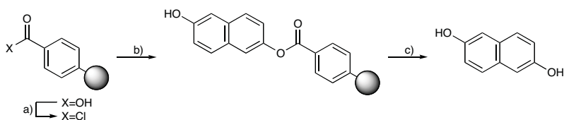
Scheme 4.5. Coupling of 2,6-dihydroxynaphthalene ( 56 ) to solid support and hydrolysis. a) Benzene, thionyl chloride. b) 2,6-Dihydroxynaphthalene, DIPEA, DMAP, CH 2 Cl 2 . c) NaOH (1 M, aq.), dioxane.
