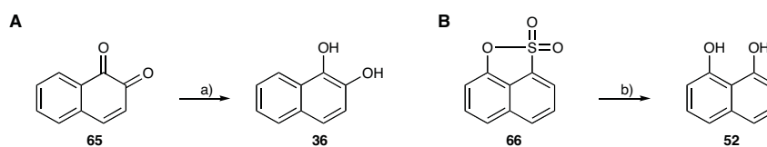
Scheme 4.7. Synthesis of 1,2-dihydroxynaphthalene ( 36 ) and 1,8-dihydroxynaphthalene ( 52 ). a) \text{NaBH}_4 , \text{EtOH} , r.t., quantitative. b) \text{KOH} , 250-300 °C, 44%. See Supplementary information for full experimental details.
