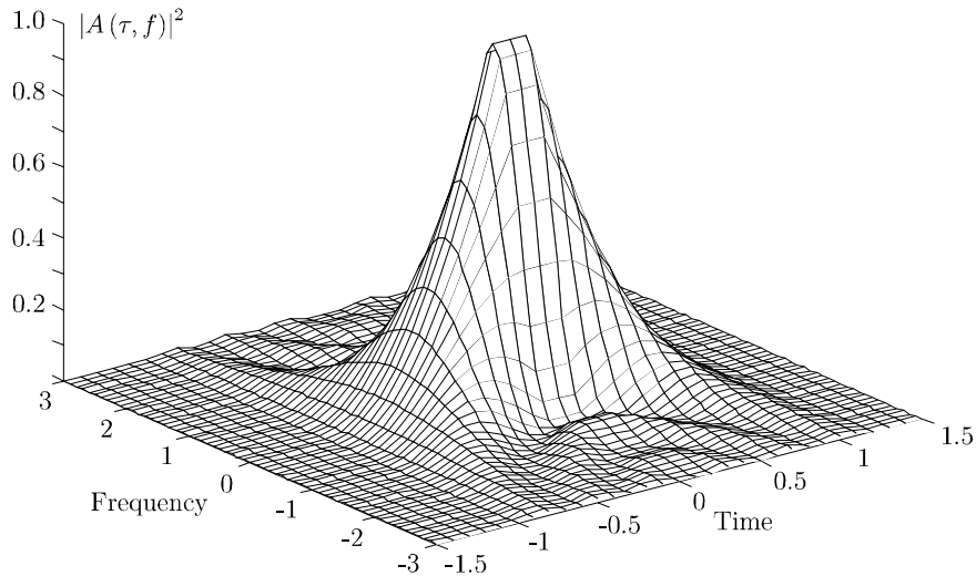
Figure A.1: Ambiguity function for a rectangular pulse and cyclic prefix with lengths \tau_0 = 1.2 and T_{cp} = 0.2 , respectively.
