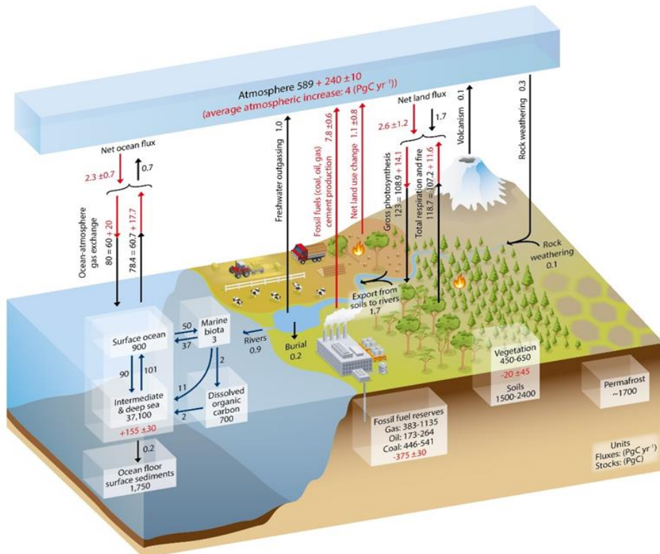
Figure 1. Global C cycle. Numbers in boxes represent reservoir mass (stocks), inventories, or storage in Petagram of C; PgC (1 Gt) and 2.1 PgC is equivalent to 1 ppm atmospheric CO 2 (Socolow and Lam, 2007). Numbers next to arrows indicate fluxes in PgC/yr. Numbers and arrows in black represent estimates of the pre-industrial so-called natural carbon cycle (ca 1750) and numbers and arrows in red represent estimates of average annual anthropogenic C fluxes (2000 - 2009). Uncertainties are reported as 90% confidence intervals. The image is from Ciais et al. (2013).
