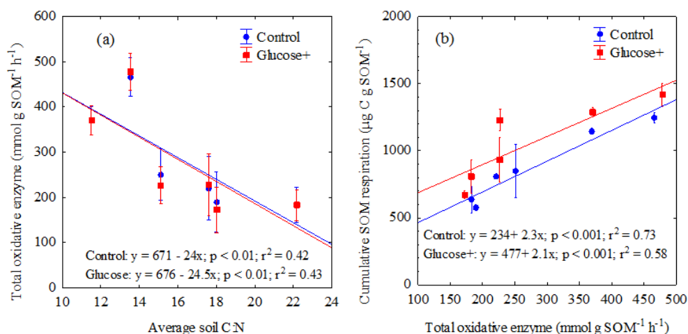
Figure 6. The relationship between total potential activity oxidative enzymes (Peroxidase+ phenoloxidase) and soil C:N ratio (a) and the relationship between SOM respiration and total potential activity oxidative enzymes (b) at the end of the one-week incubation period. Error bars represent standard error of the mean. Figure from Paper III.
