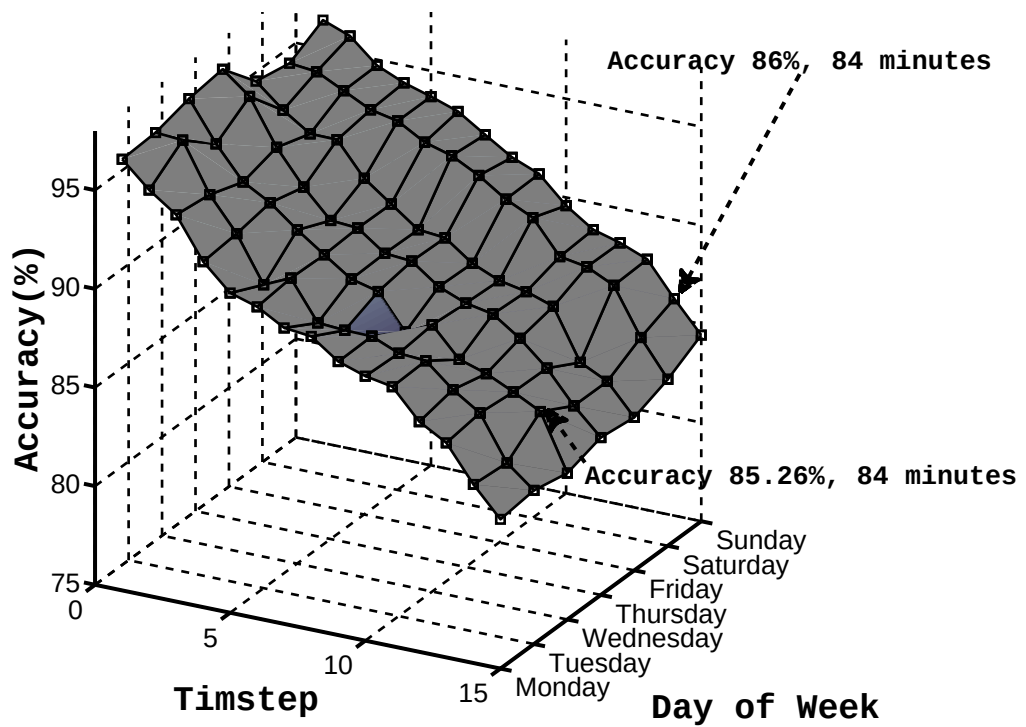
Figure 3: M4 motorway westbound prediction
