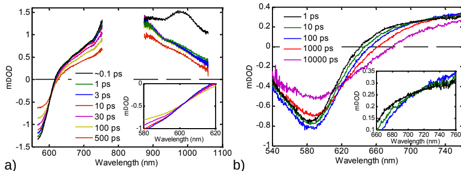
Figure 4.7. Transient absorption spectra of a) APFO15:PCBM and b) APFO3:PCBM blend samples. The observed isosbestic points are highlighted in the insets.
