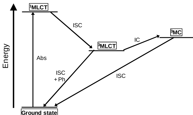
Figure 5.3. A Jablonski diagram illustrating the most important states and photoinduced processes in \text{Ru}^{\text{II}} -polypyridyl complexes. Most experimental lifetime studies do not consider the ^1\text{MLCT} - ^3\text{MLCT} transition as most of the photophysical processes occur from the ^3\text{MLCT} state.
