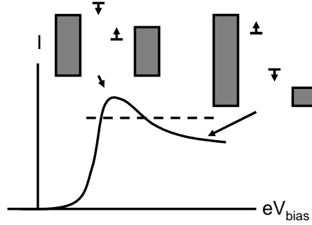
Figure 6.4: Sketch of the level renormalization described in Ref. [69] for large Coulomb interaction, see also Eq. (6.12). The arrows indicate how the levels move relative to the chemical potential of the nearest lead, and the dashed line indicates the plateau value of the current in case of no level renormalization. First the level renormalization gives a decrease of the detuning between the levels, causing an overshoot of the current as compared to the plateau value. This is followed by an increased detuning causing a significant negative differential conductance. See in particular Fig. 6.5d for \Delta = \Gamma/4 .
