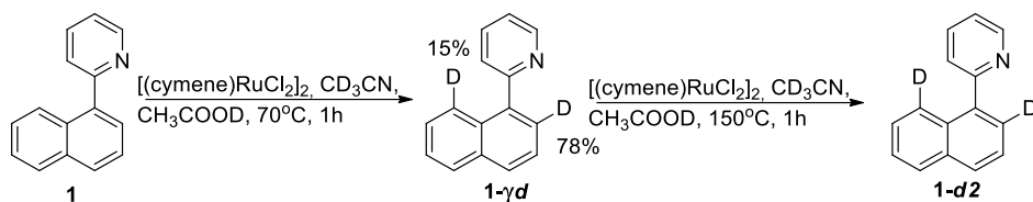
Scheme 17. Ru-catalysed D-exchange.
