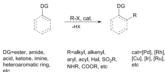
Scheme 1. General description of the ligand-directed C—H activation.
