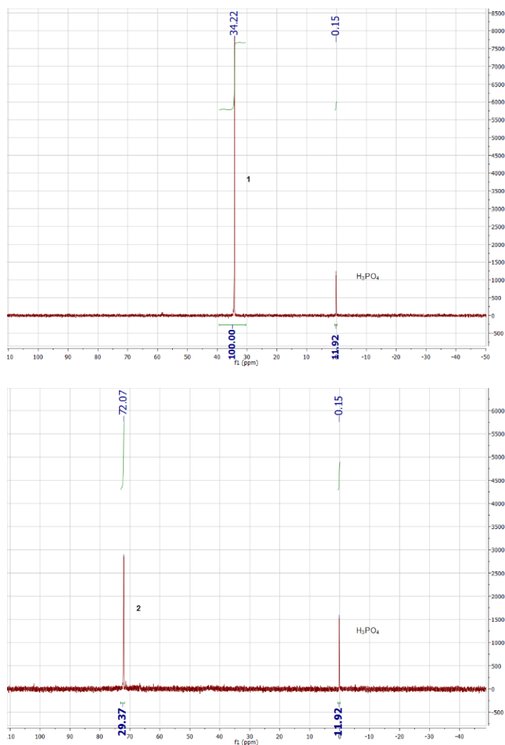
Figure 1. Representative ^{31}\text{P} NMR spectra before the addition and 10 minutes after the addition of [\text{Pd}] .
