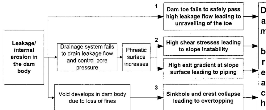
Figure 2. Failure mechanisms initiated by internal erosion in the embankment dam (from Nilsson and Bartsch 2004).
