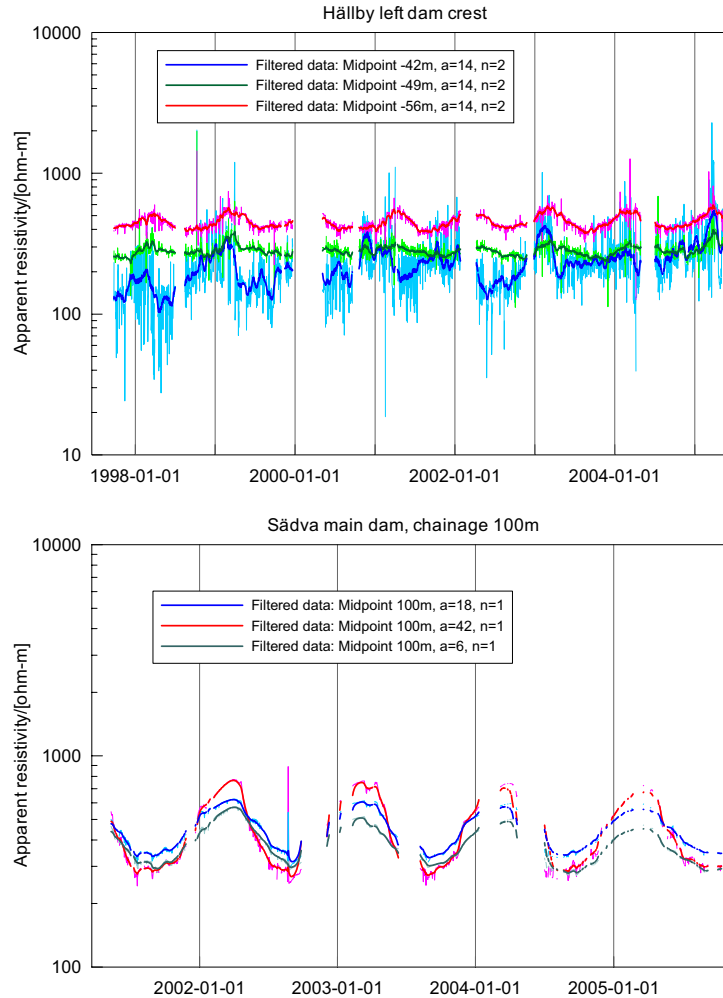
Figure 17. Example of time-series of apparent resistivities (thin lines) with filtered data from long-term measurements at the Hällby (top) and the Sädva (bottom) dams.
