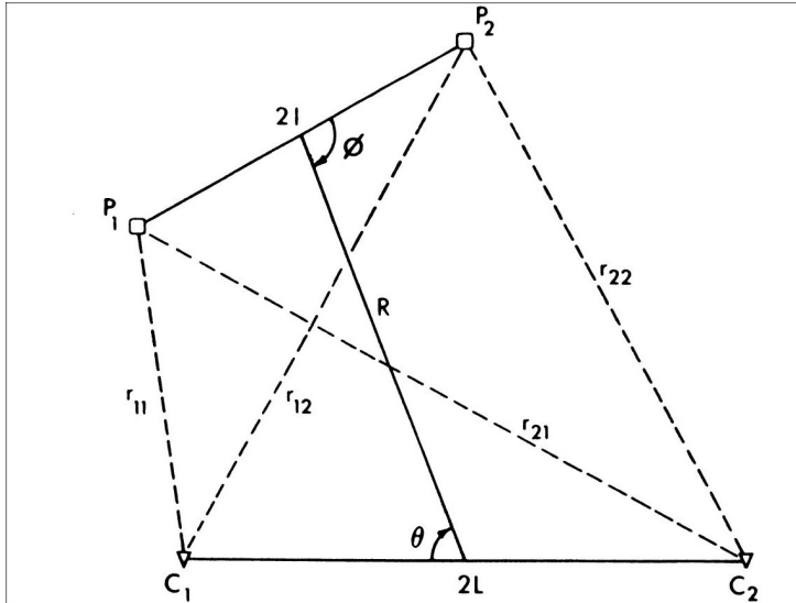
Figure 6. Sketch of the arrangement of a general four-electrode measurement with potential electrodes P1, P2 and current electrodes C1, C2 ( 0 < \theta, \phi < \pi ). The distances between the electrodes are used to calculate the geometric factor, K (from O'Neill and Merrick 1984).
