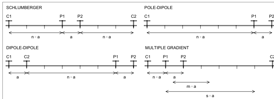
Figure 9. Common arrays used in resistivity surveys and their descriptions using a-spacing and n-factors. In general a is the distance between the potential electrodes and n \cdot a is the closest distance between a current and a potential electrodes. Wenner array is the special case when n=1 in the Schlumberger array. The multiple gradient array is a bit more complicated to explain in these terms; n \cdot a is the relative distance between the closest current electrode to the potential dipole being negative if the dipole is closer to the second current electrode m \cdot a is the distance between the midpoints of the current and potential electrode pairs, and the separation factor s indicates the maximum number of potential dipoles with internal distance a that can be distributed in the array.
