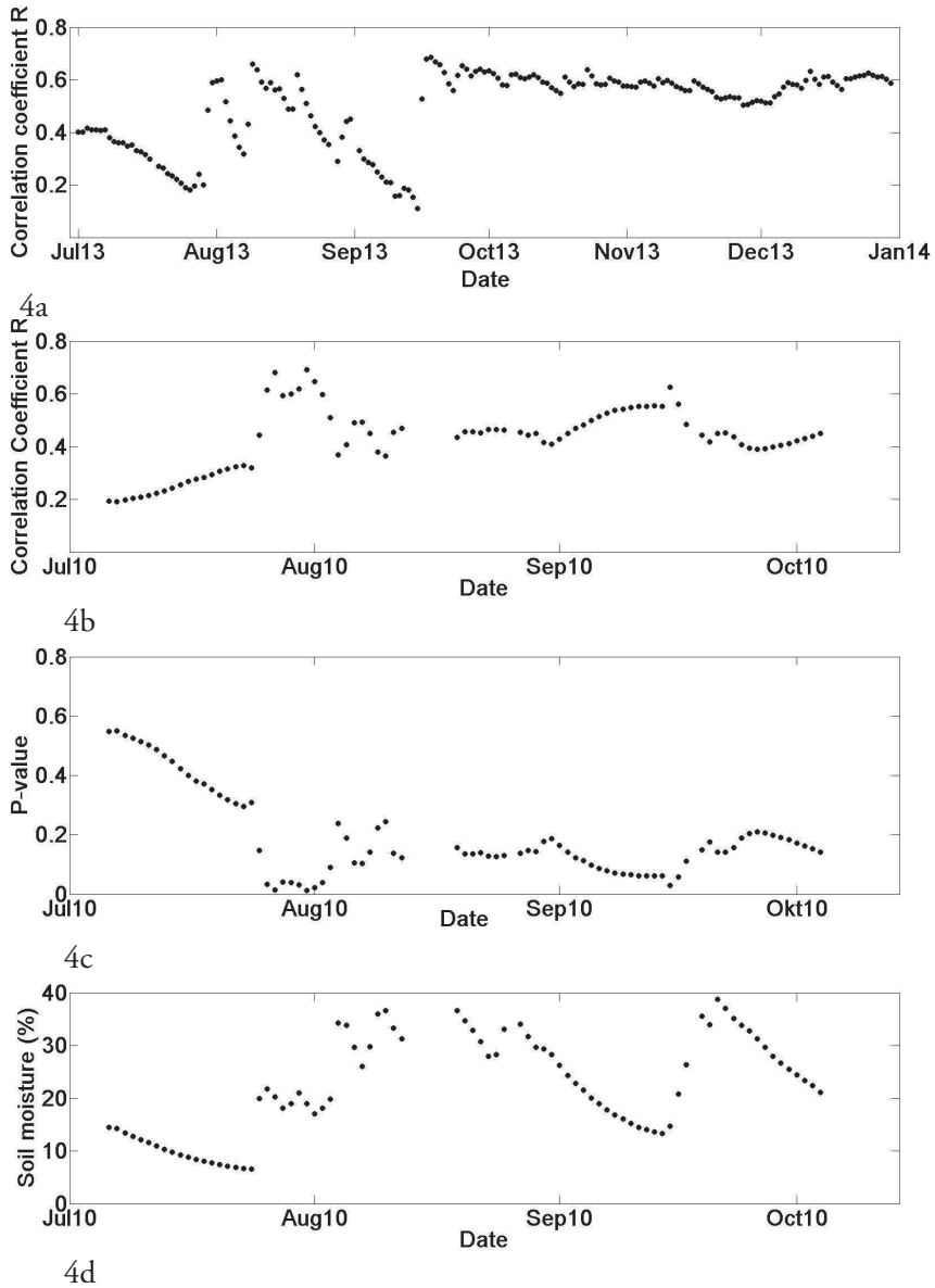
Figure 4. Daily correlation between TWI and soil moisture measured at a) 9 locations July- December 2013; b) 12 locations July-October 2010; c) daily significance level for correlations between TWI and soil moisture measured at 12 locations July-October 2010; and d) daily soil moisture for the time period July-October 2010.
