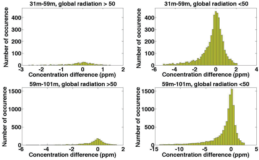
Figure 3. Occurrence of \text{CH}_4 concentration differences for different height intervals and for day and night. Data between the 2nd and 98th percentiles are shown.
