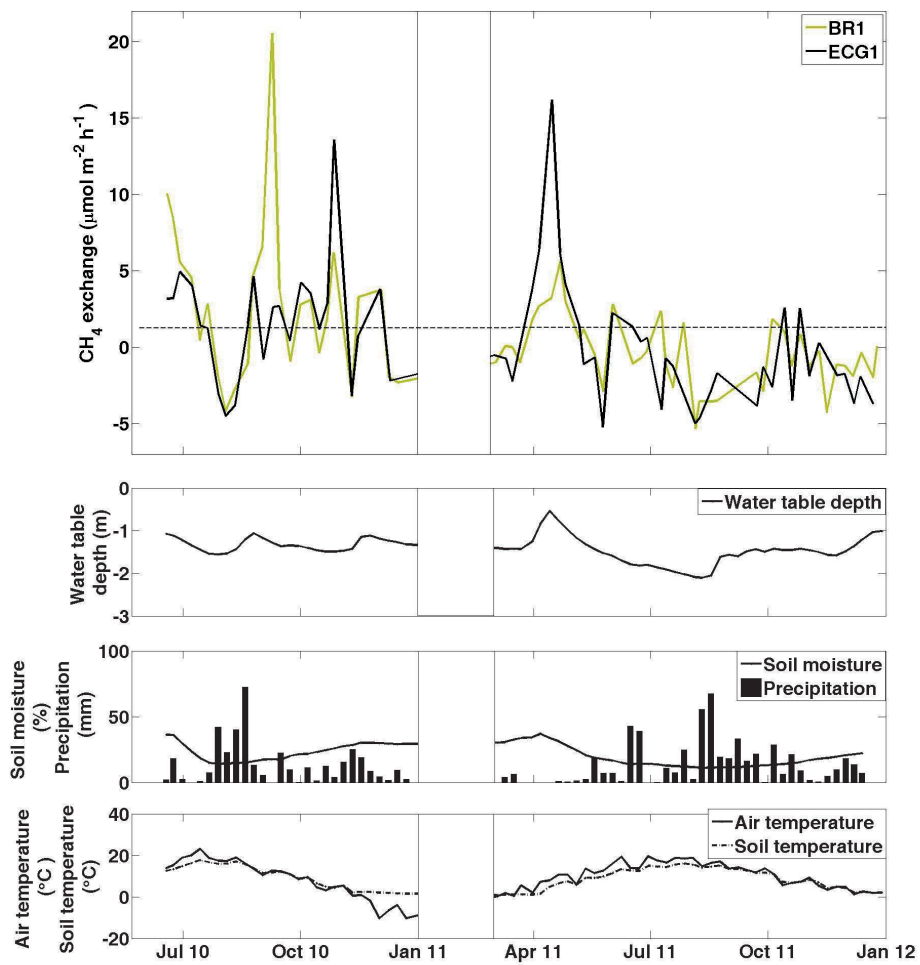
Figure 8. Weekly mean values of \text{CH}_4 exchange, water table depths, soil moisture, precipitation, air temperature and soil temperature.
