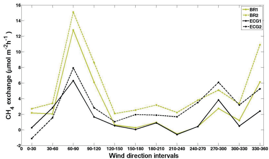
Figure 6. Average \text{CH}_4 exchange for wind directions binned in 30 degrees intervals.
