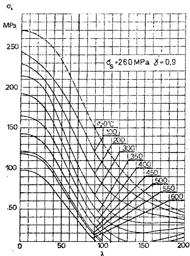
Figure 11. Variation with the steel temperature \vartheta_s of the relationship between the buckling stress \sigma_k and the equivalent slenderness ratio \lambda for fire exposed, axially compressed steel columns, partially restrained to longitudinal expansion and made of steel with a yield point stress at ordinary room temperature \sigma_s = 260 MPa
