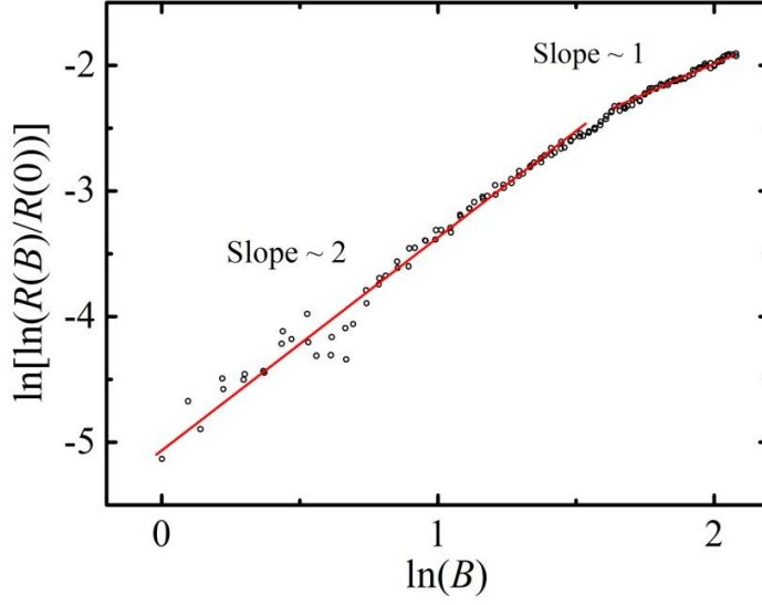
Figure 7.12: Log-double log plot of the resistance versus magnetic field for a single \text{Ga}_{1-x}\text{Mn}_x\text{As}:\text{Zn} NW ( x = 0.1\% ) at 1.6K, clearly showing a quadratic dependence at low magnetic field strengths and a weaker linear dependence at high magnetic field strengths.
