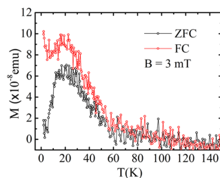
Figure 4. Temperature-dependent ZFC and FC magnetization curves of Mn implanted GaAs nanowire ensembles at an applied magnetic field of 3 mT applied perpendicular to the substrate surface with deposited NWs.
