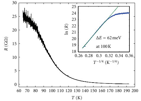
FIGURE 2: \text{Ga}_{0.95}\text{Mn}_{0.05}\text{As} nanowire resistance as a function of temperature. The inset shows a plot of \ln(R) versus T^{-1/4} , with the extracted activation energy of 62 meV at 100 K.
