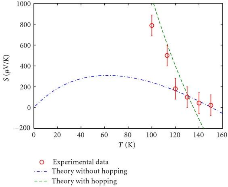
Figure 6.12: Thermopower for a single \text{Ga}_{1-x}\text{Mn}_x\text{As:Zn} ( x = 5\% ) NW device of 40 nm diameter, as a function of temperature. The experimental data matches well at high temperatures with values calculated using a model without hopping [89]. Below 120 K, the nanowire thermopower deviates strongly from the model without hopping. Addition of a hopping term qualitatively accounts for the rise in thermopower [4].
