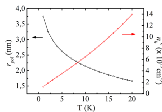
Figure 3. Black curve shows the theoretical estimate of the polaron radius obtained from eq 1. Red curve shows the critical hole density versus temperature, defined as the density satisfying the magnetic percolation transition condition given in eq 2 at a given temperature.
