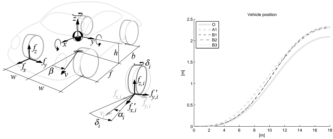
Figure 3: Left: Vehicle model with notation; Right: Resulting optimal vehicle path for maximum displacement maneuver (O - FWS, A1 - AWS, B1 - AWD, B2 - FWD, B3 - RWD).
