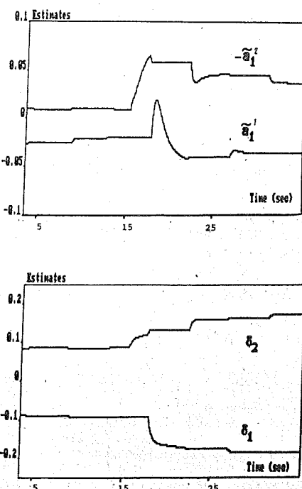
Fig. 6. Time histories of estimates \hat{\delta}_1 , \hat{\delta}_1^2 , \hat{\delta}_2 , and \hat{\delta}_2 under friction variations.
