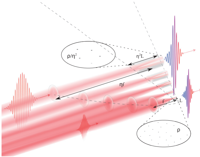
Figure 2.10: Illustration of the scale invariance of the HHG process. The lowest laser beam represents the un-scaled process with gas density \rho , focal length f and gas medium length L . The size of the laser pulse represents the input pulse energy E_{\text{in}} . The laser beam with the increased laser pulse size represents an increased input pulse energy \eta^2 E_{\text{in}} with scaled parameters \rho/\eta^2 , \eta f and \eta^2 L . The conversion efficiency of the process is unaffected ( \Gamma \rightarrow \Gamma ), thus the output pulse energy scales with the input energy ( E_{\text{out}} \rightarrow \eta^2 E_{\text{out}} ). (Image courtesy of C. Heyl.)
