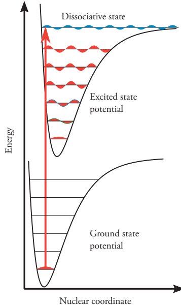
Figure 1.1: Illustration of the Franck-Condon principle.
