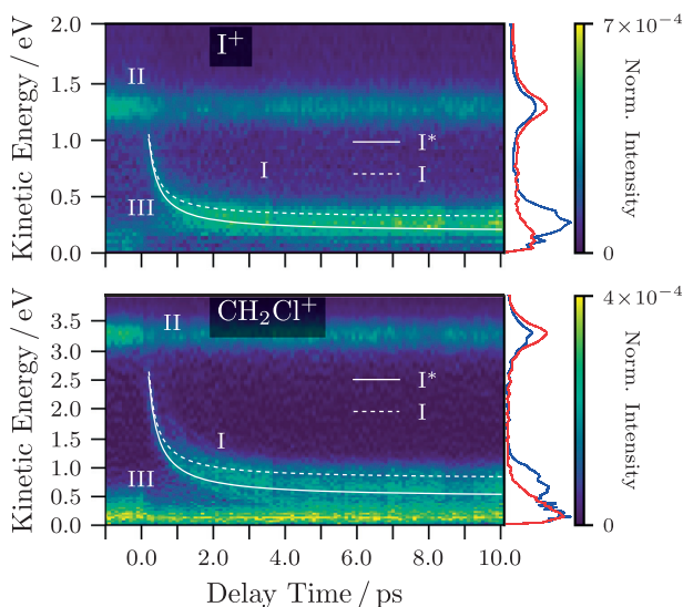
Figure 4.20: Kinetic energy spectrogram of \text{I}^+ ions (top) and \text{CH}_2\text{Cl}^+ ions (bottom), obtained from Abel-inverted momentum distributions. One time-dependent (I) and two static (II and III) channels are clearly visible for both fragments. Simulated curves for dissociation pathways leading to the ground state \text{I}(^2\text{P}_{3/2}) (dashed) and to the spin-orbit excited state \text{I}^*(^2\text{P}_{1/2}) (solid) are drawn in white. (Reproduced from Paper VI.)
