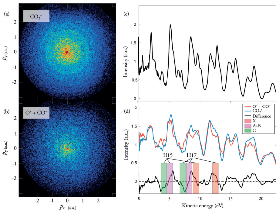
Figure 4.23: Photoion-photoelectron covariance results from photoionization of \text{CO}_2 . (a) and (b) show photoelectron momentum maps in covariance with \text{CO}_2^+ and \text{O}^+ + \text{CO}^+ photoions, whose TOF spectra were recorded. The photoelectron spectrum calculated from the VMI data is shown in panel (c). (d) The covariance maps in (a) and (b) were Abel-inverted and angularly integrated to obtain the photoelectron covariance shown in red ( \text{O}^+ + \text{CO}^+ ) and blue ( \text{CO}_2^+ ). The calculated difference spectrum is displayed in black. The assigned contributions from the X, A+B and C states are indicated for photoelectrons produced by photons from harmonic orders 15 and 17.
