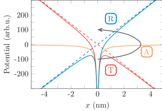
Figure 2.5: Illustration of the three-step model: The external electric field of the laser pulse distorts the atomic potential to such an extent, that one or more electrons can escape the potential via tunnel ionization, depicted in red (T). Once an electron escapes the atomic potential, it is accelerated in the laser field (orange, (A)). When the sign of the field flips, the electron is decelerated and its direction of motion is reversed. Under favorable conditions, the electron can recombine with the parent atom (blue, (R)), while emitting a photon. The energy of the photon corresponds to the energy imparted to the electron by the laser field plus the ionization potential of the atom.
