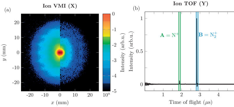
Figure 4.1: Photoion dataset synchronously acquired with the DVMIS using \text{N}_2 molecules as target gas. (a) The ion VMI image, where the left half represents the integrated detector image, and the right half the Abel-inverted image. (Reproduced from Paper V.) (b) The acquired ion TOF spectrum. The time windows used for the covariance analysis are indicated in green ( \text{N}^+ ) and blue ( \text{N}_2^+ ).
