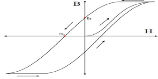
Figure 1. Typical magnetization curve for ferromagnetic materials.
