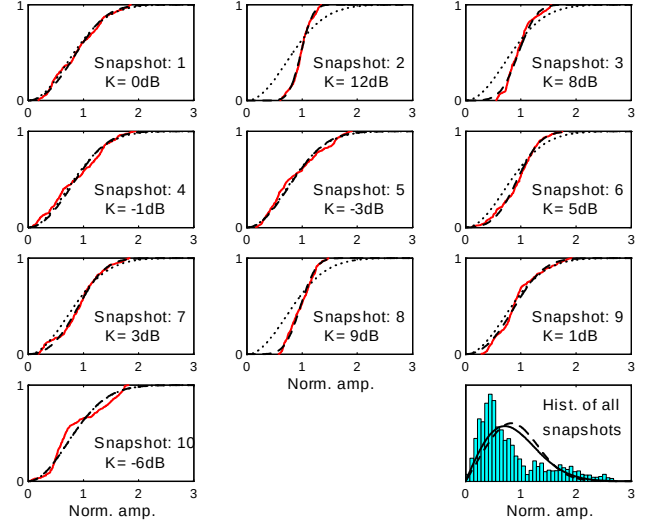
Fig. 6. Cdf:s of the amplitude statistics for each snapshot of measurement Tx3 to Rx9, rotation 1, using antenna elements t1 to r3. The solid lines are measured data, the dashed lines are best fit Riceans (with the K-factor printed in the figure), while the dotted lines are best fit Rayleighs. It is clearly seen that different snapshots have different distributions.
