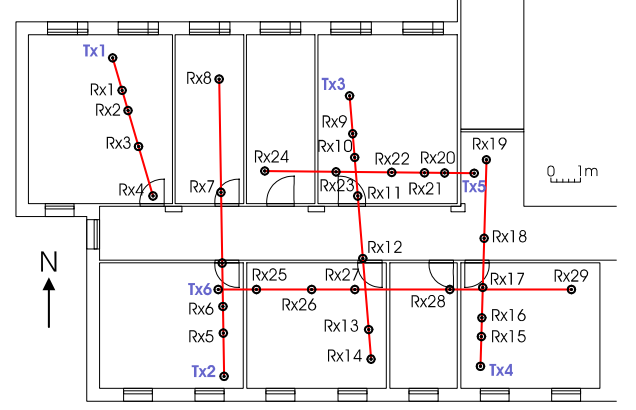
Fig. 2. Site map of the measurement positions for the static scenario. Measurements were only made between positions along the same line.
