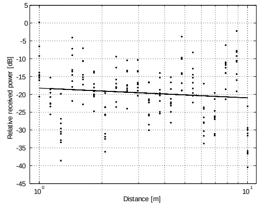
Fig. 4. Scatter plot of the received power vs. distance for all LOS measurements. For each value of the distance d , there are nine measurement points, corresponding to the different Tx and Rx orientations as described in Section II. The best fit regression line corresponds to a pathloss exponent n = 0.27 .
