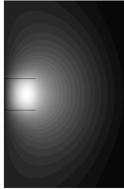
Figure 8.14: The electric field of the lowest resonant frequency f_r = 46.2 GHz for the cylindric resonator with \epsilon = 10 , radius a = 1 mm and height h = 1 mm. The mode is a TE-mode, i.e., the electric field is directed along the azimuthal direction.
