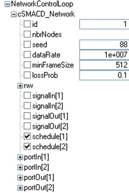
Figure 5: Simulation variables
