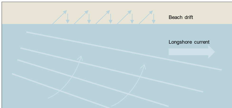
Figure 2.3 Schematic picture of longshore sediment transport due to longshore current and swash processes.
