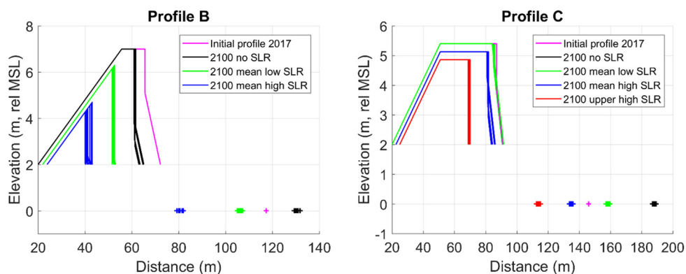
Figure 5.5 Simulated beach–dune evolution for Profile B and C. The '+' indicates intersection with MSL.
