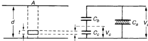
Figure 3: Electrical discharge in a cavity and its equivalent circuit [3].
