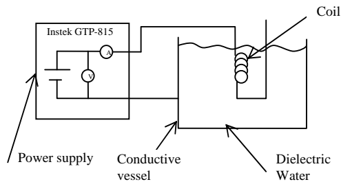
Figure 9: Schematic view of the electrical test setup.
