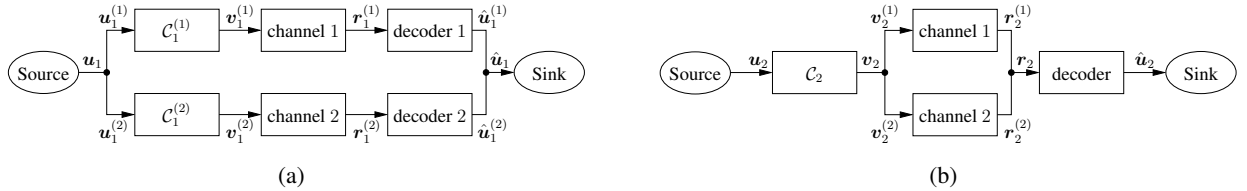
Fig. 1. Transmission scheme \mathcal{T}_1 (a) and \mathcal{T}_2 (b) with two parallel, independent channels.
