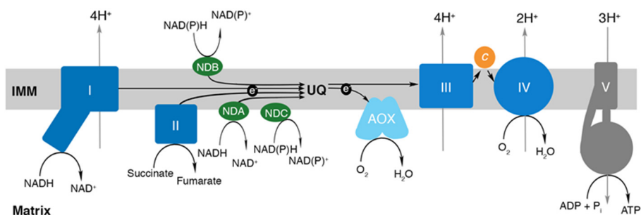
Figure 3. Schematic representation of oxidative phosphorylation in plants.
