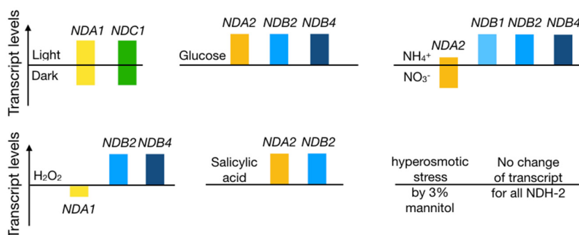
Figure 11. Transcription changes of NDH-2 to different conditions
