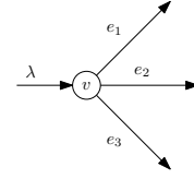
Fig. 4: A local network with \mathcal{E}_v^+ = \{e_1, e_2, e_3\} .
