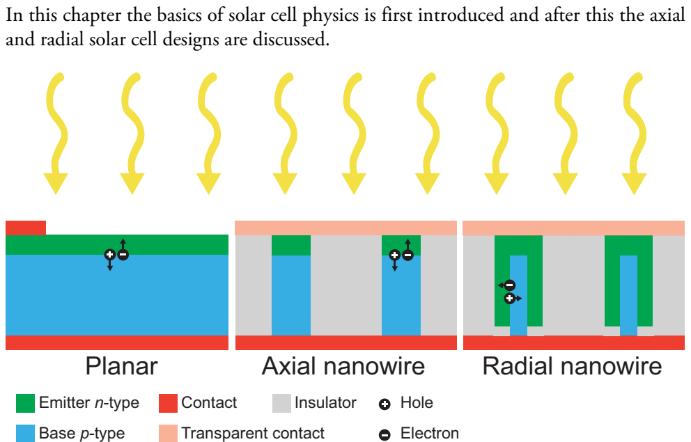
Figure 4.1 Principal structure of a conventional planar, axial nanowire and radial nanowire solar cell. An axial nanowire solar cell is analogous to a planar since charge separation and light propagation occurs in the same direction. In a radial nanowire solar cell charge separation instead occurs orthogonal to the direction of light propagation.
