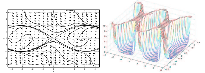
Figure 2: Left: Phase plot for pendulum with energy control. Right: Graph of the density function 1/E^2 .
