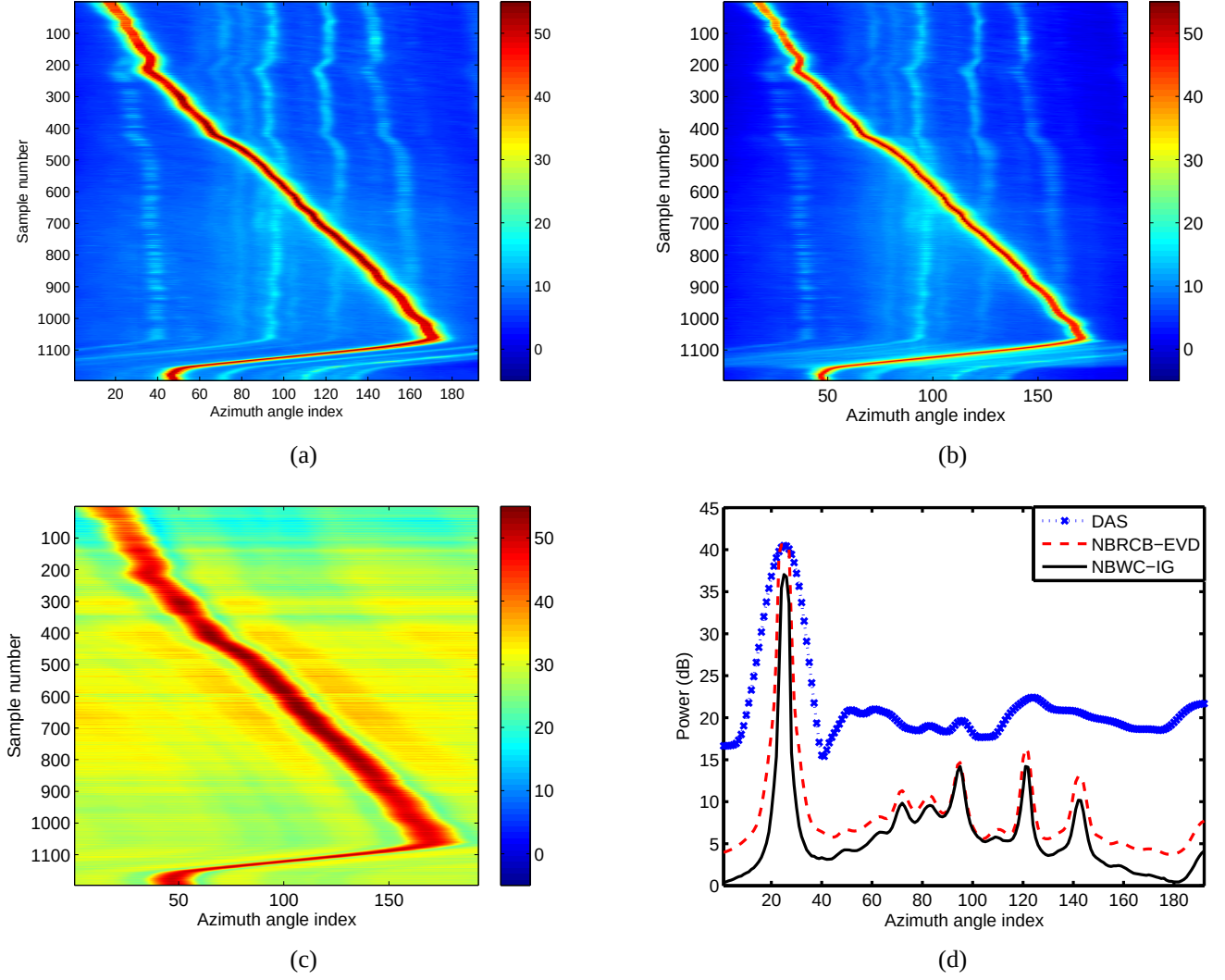
Fig. 3. For the strong controlled source run, bearing time records with K = 80 for (a) NBRCE-EVD, (b) NBWC-IG, (c) SDAS. For sample 75, (d) the azimuth spectra.
