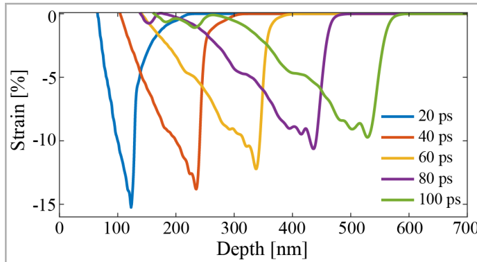
Figure 6.2: Evolution of strain waves in graphite after laser excitation with a fluence of 300 mJ/cm 2 .
