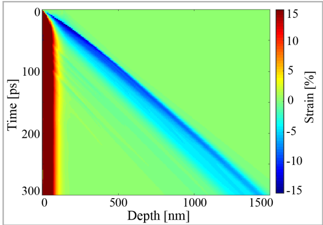
Figure 5.16: Evolution of strain in graphite with a laser fluence of 300 mJ/cm 2 .
