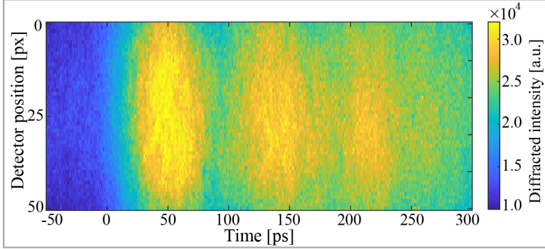
Figure 3.17: X-ray diffraction signal acquired with an X-ray streak camera.
