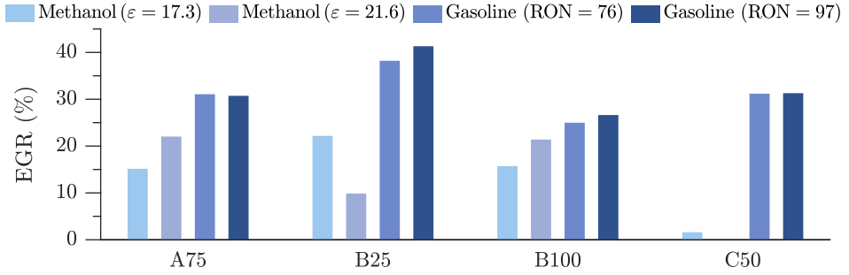
Figure 5.7: EGR for all operating points, comparing methanol (with \varepsilon = 17.3 and \varepsilon = 21.6 ) and gasoline (with RON = 76 and RON = 97).
