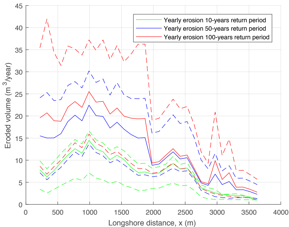
Figure 10. Estimated eroded volume (solid lines) together with the upper and lower limit of the 95% confidence intervals derived with profile likelihood method.
