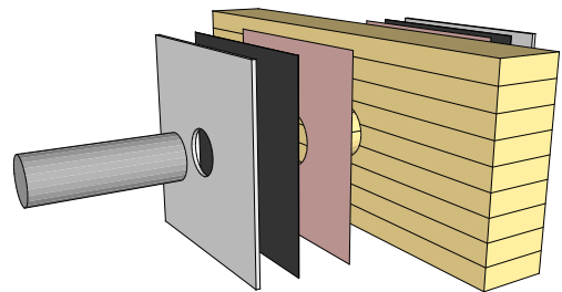
Figure 1: Exploded view of the shear plate dowel joint (SPDJ).
