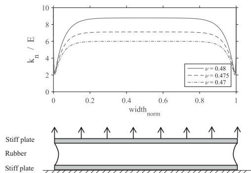
Fig. 6. Stiffness variation determined by numerical tension simulation of a rubberlike material. The specimen width is 30 times the rubber layer thickness. The rubber layer is modelled using an isotropic linear elastic material with E = 3.6 MPa.
