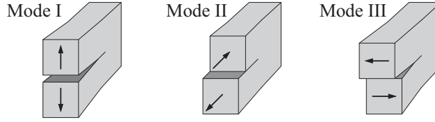
Figure 3.4: The three fundamental modes of fracture deformation. From Danielsson [39].
