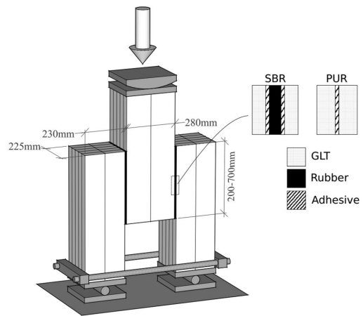
Fig. 1 Double lap joint test setup
