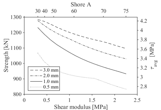
Figure 10: Failure strength of the SPDJ reference design for increasing stiffness using different rubber layer thicknesses. Stiffness is given in Pascal (lower x-axis) and Shore A (upper x-axis).
