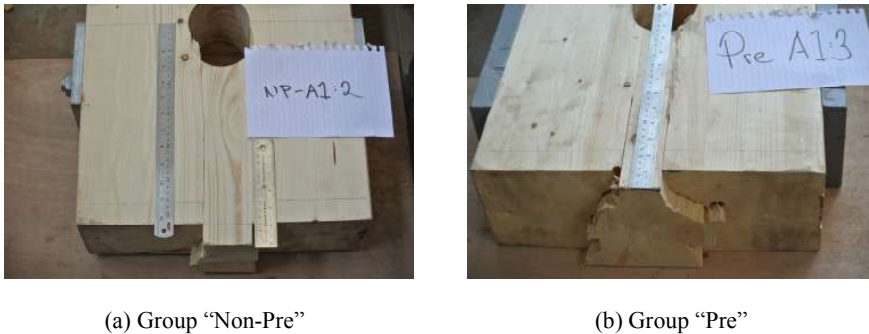
Figure 6: Failure modes of SLDDCs with lateral reinforcement
