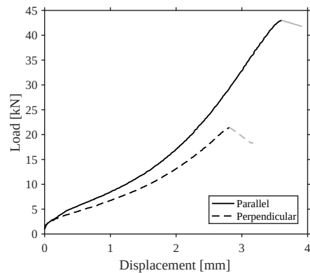
Figure 6: Typical load-displacement curve for short term testing of SPDJ specimens loaded parallel and perpendicular to grain. Grey lines are very fast failure propagation and should thus be considered brittle.
