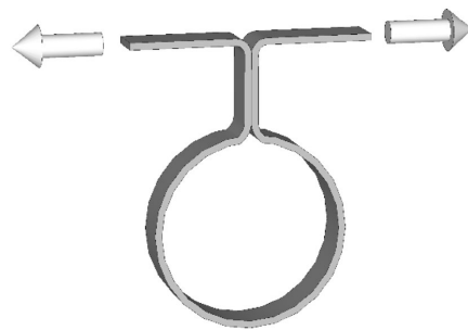
Fig. 2 Rubber-adhesive adhesion tensile test. Bonded area was 50×50 mm 2
