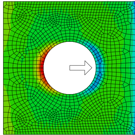
(b) Distribution of normal stresses perpendicular to grain. Colour limits are -6 MPa (blue) and 6 MPa (red, peel stress). Green represents zero stress.
