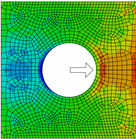
(a) Shear stress distribution. Colour limits are 3.5 MPa (blue) and 6.5 MPa (red). Green represents a stress of 5 MPa.
