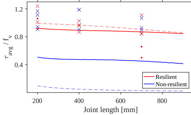
Figure 4.6: Numerical results (lines) of experimental setup compared to experimental data (markers). Wood failure close to the bond line is marked with \times while dots mark premature adhesion failures. The solid lines are numerical FE results while the dashed lines are analytical results according to Volkersen theory, using shear strength f_v = 4.4 MPa.
