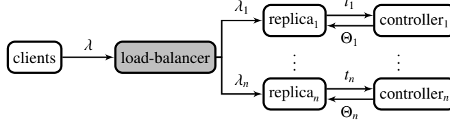
Figure 1: Architecture of a brownout cloud service featuring multiple replicas.
