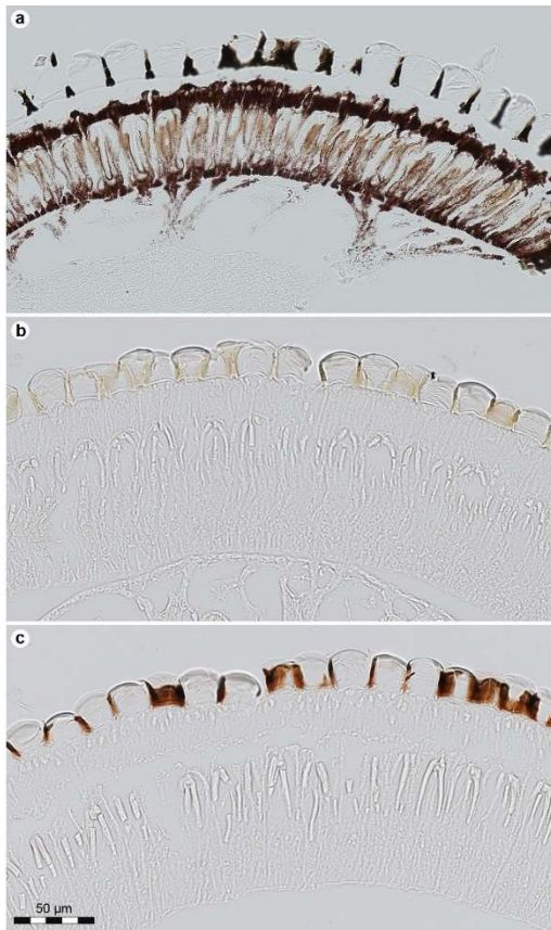
Extended Data Figure 9 | Histological sections through Nephrotoma suturalis compound eyes stained with Fontana-Masson. a , Untreated section. b , Section bleached with hydrogen peroxide. c , Bleached section stained with Fontana-Masson. Note darkening of the corneal cuticle in the facet walls, indicating presence of melanin. Images are representative of three independent experiments.
