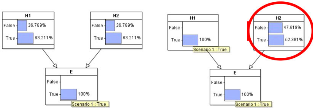
FIG. 4. Bayesian network with HH-incoherence.
