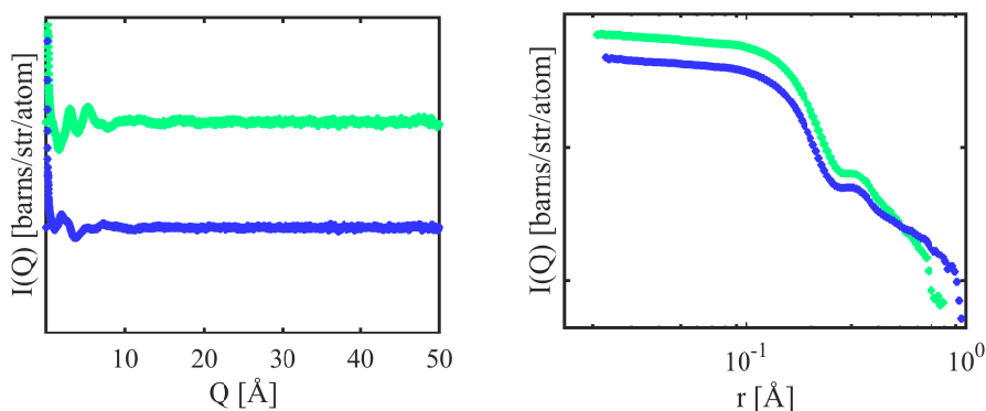
Figure 3.4: The scattering pattern of a 0.4M C_{10}TABr with 22 wt% silica salt. Left: displayed on a linear scale for near to intermediate Q -range. Right: displayed on a logarithmic scale for low Q -values, highlighting the micelle contribution.
