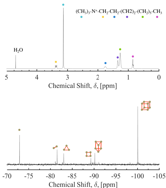
Figure 3.2: Two different NMR spectra; (top) ^1\text{H} spectrum of \text{C}_{10}\text{TABr} in \text{D}_2\text{O} , (bottom) ^{29}\text{Si} spectrum of a silica salt solution (18wt%). The different hydrogens in the surfactant have been marked in the spectra, and an example of peak splitting can be seen at the pink dot. The different silica species are marked in the spectrum, with silicon atoms marked as beige dots, all linked by oxygens. The ^1\text{H} spectra has been recorded for a few seconds (16 pulses), whereas the the silicon spectra has been recored for over 3 hours (128 pulses). The concentration of the protons are much higher than that of the silicon atoms; one surfactant molecule contains 21 protons whereas the largest silica specie only contain 8 Si atoms. This will also contribute to the difference in the signal-to-noise between the two spectra.
