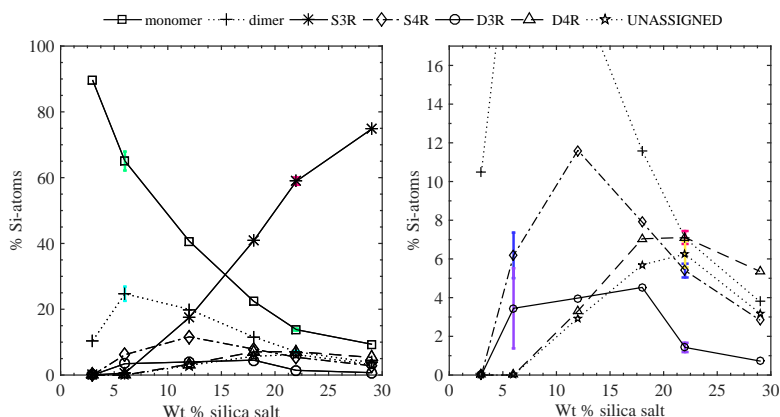
Figure 4.3: The concentration dependence of the different silica species with increasing silica salt concentration. The error bars for two of the concentrations show the variation between different experiments on equivalent samples. The concentration is given as the number Si atoms in one type of specie in relation to the total number of Si atoms in the solution.
