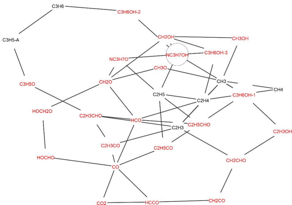
Figure 8. A skeletal mechanism, ACR95, containing 39 species and 95 reactions for high temperature ignition of n-propanol ( NC_3H_7OH ) and air. Only carbon containing species have been included for clarity, and species containing at least one oxygen atom have been coloured red. A line between two species indicates that at least one reaction connects the two.
