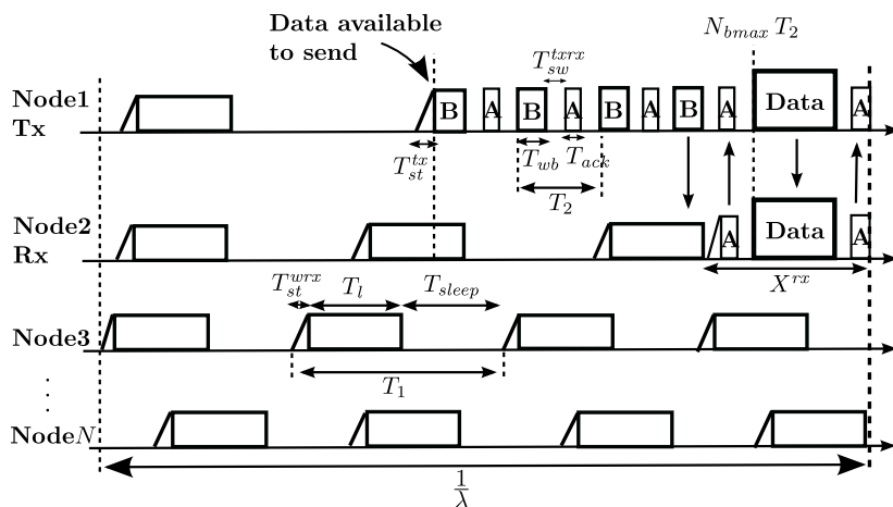
Figure 5: DCW-MAC scheme.
