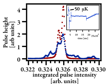
Figure 4.31. Pulse height spectrum of ^{55}\text{Fe} emission data using artificially introduced temperature fluctuations of up to \pm 50\ \mu\text{K} shown in the inset before (blue line) and after correction red (red line).
