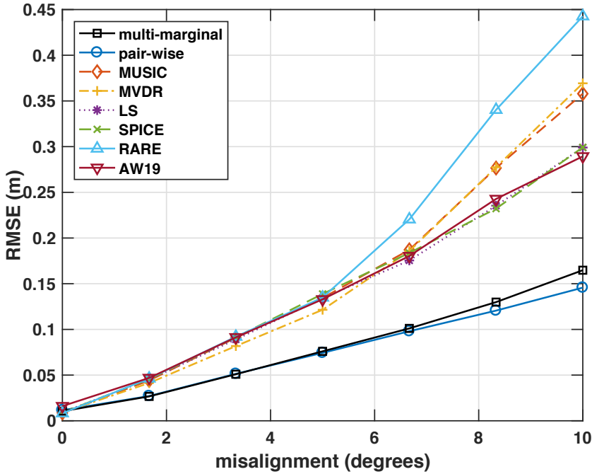
Figure 9: Error in location of spectral peaks, as function of the misalignment angle.
