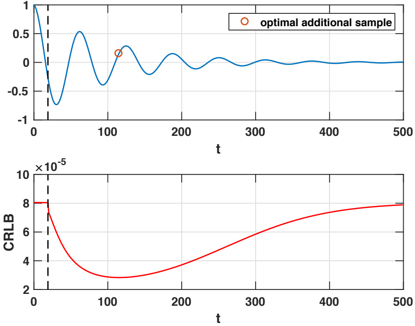
Figure 6: The problem of collecting one additional sample from (6) after having sampled at t = 0, 1, \dots, N_{\text{initial}} - 1 , with N_{\text{initial}} = 20 . Top panel: real part of (noise-free) waveform. Bottom panel: CRLB for decay parameter \beta as a function of the additional sample collected.
